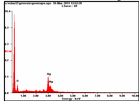
Fig 4. EDAX of Silver nanoparticles
