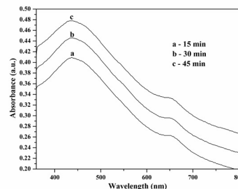
Fig 1a. UV-vis spectra of Silver colloid
