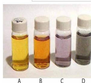
Fig 1. Colloidal silver in various stages of aggregation, (A) clear yellow sol, (B) dark yellow sol, (C) violet sol, and (D) grayish sol, as aggregation proceeds.
