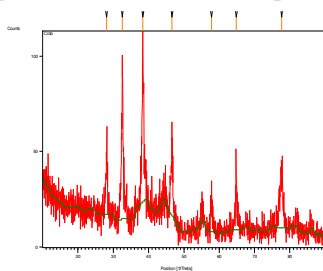
Fig 5. XRD pattern of silver nanoparticles.
